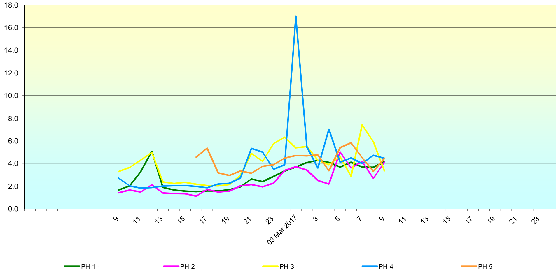
Channel: Benzene (ug/m3), period: 02 Mar 2017-03 Mar 2017 - Raw data
