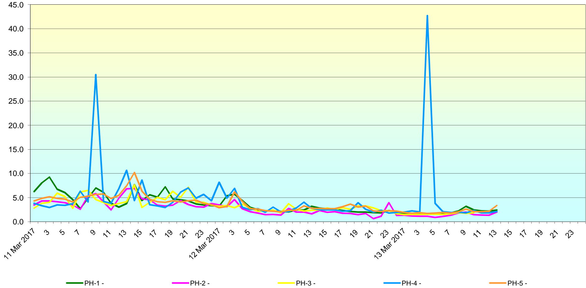
Channel: Benzene (ug/m3), period: 11 Mar 2017-13 Mar 2017 - Raw data
